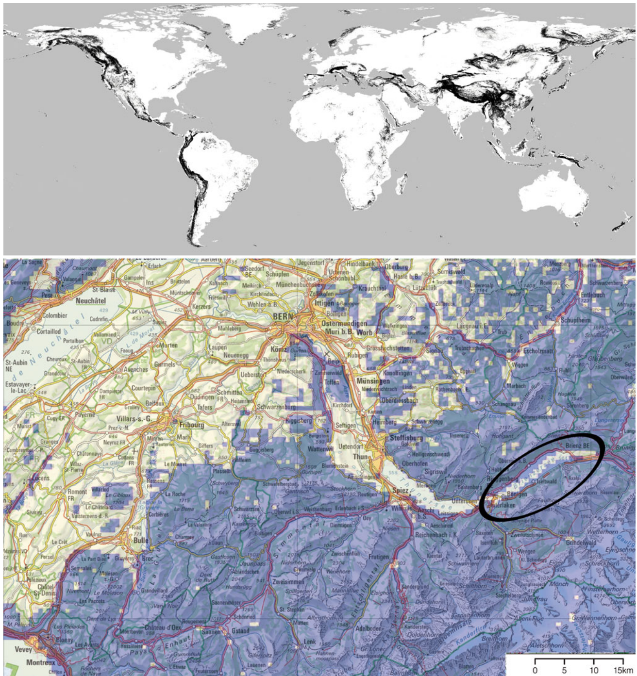
Fig. 1 Top Mountain area according to our ruggedness definition (elevational distance >200 m between nine 30'' pixels) on the global scale ( black , non-rugged terrain in white ). Below Mountain area on the regional scale ( blue , non-rugged terrain in yellow ). The below map shows a part of Switzerland from Neuchâtel to Grindelwald
